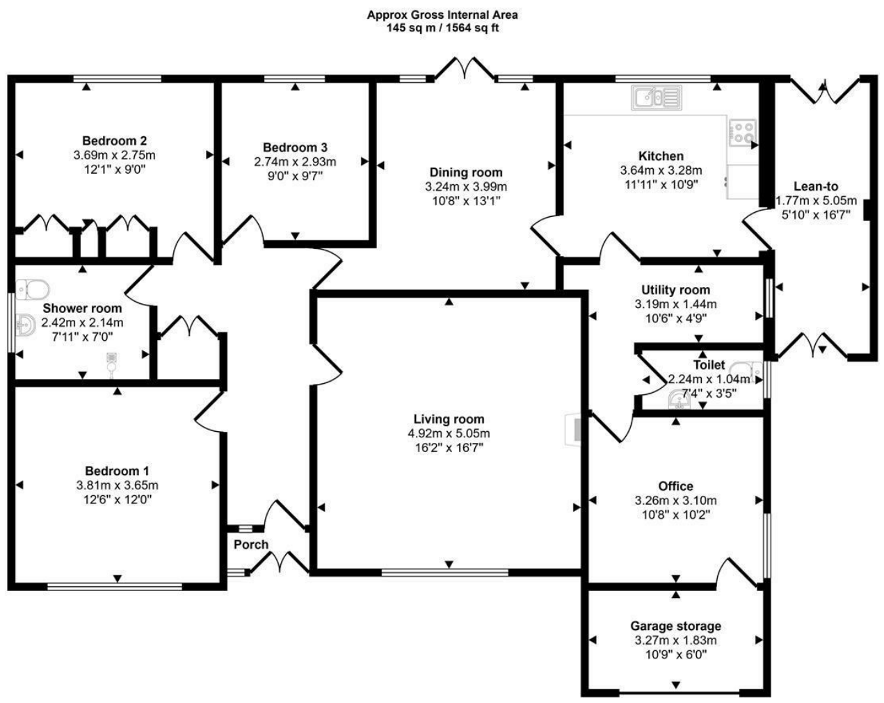
Floorplan
